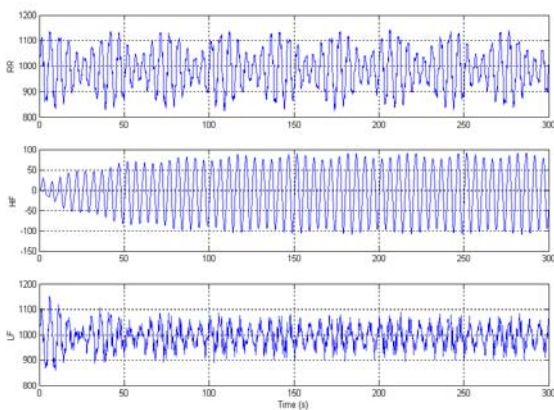
Fig. 7 Adaptive filter outputs for Simulation B
